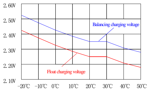
Charge voltage Vs ambient temperature curve
